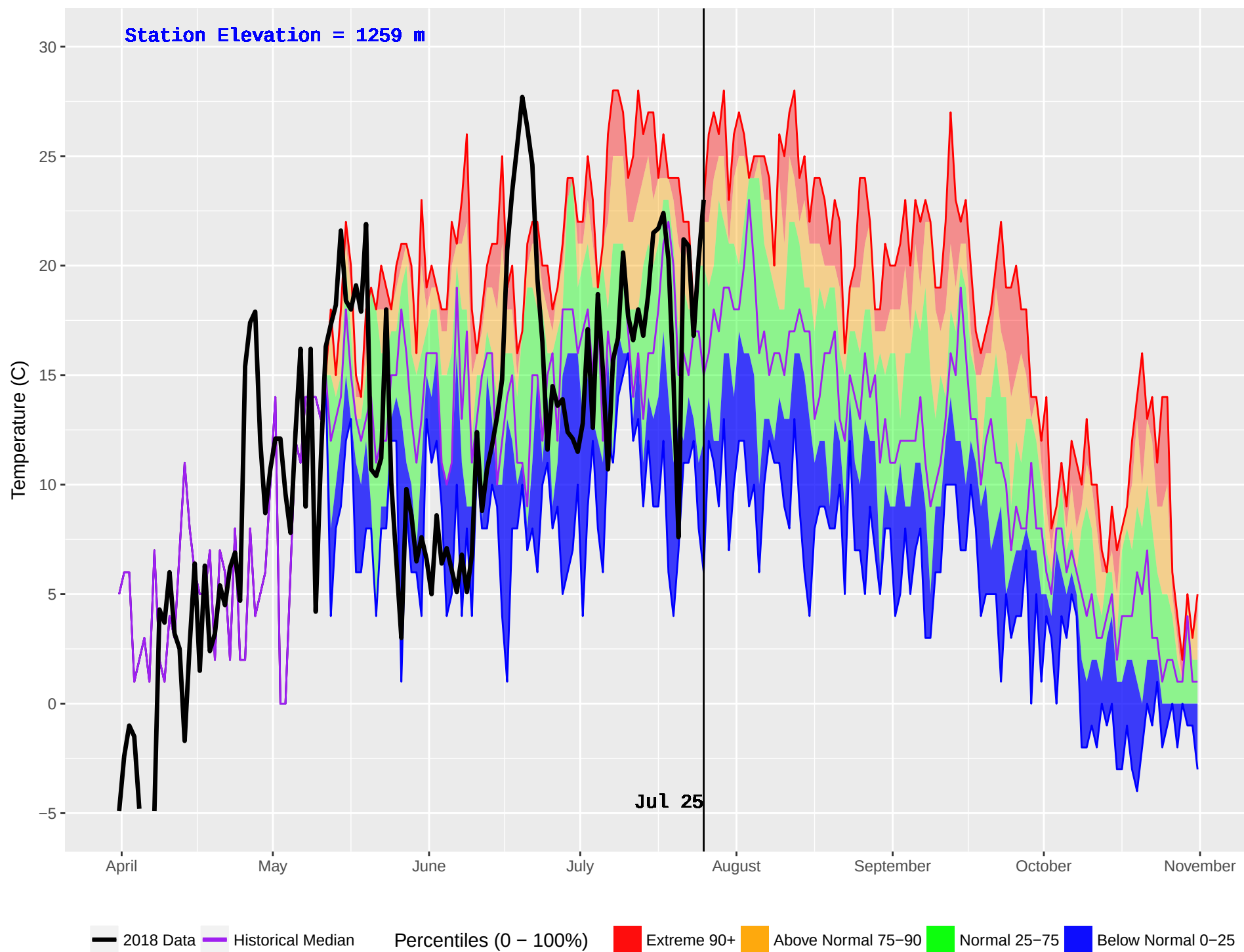
PARROTT (183) : Historical (1995–2016) and Current (2018) Noon Temperature
