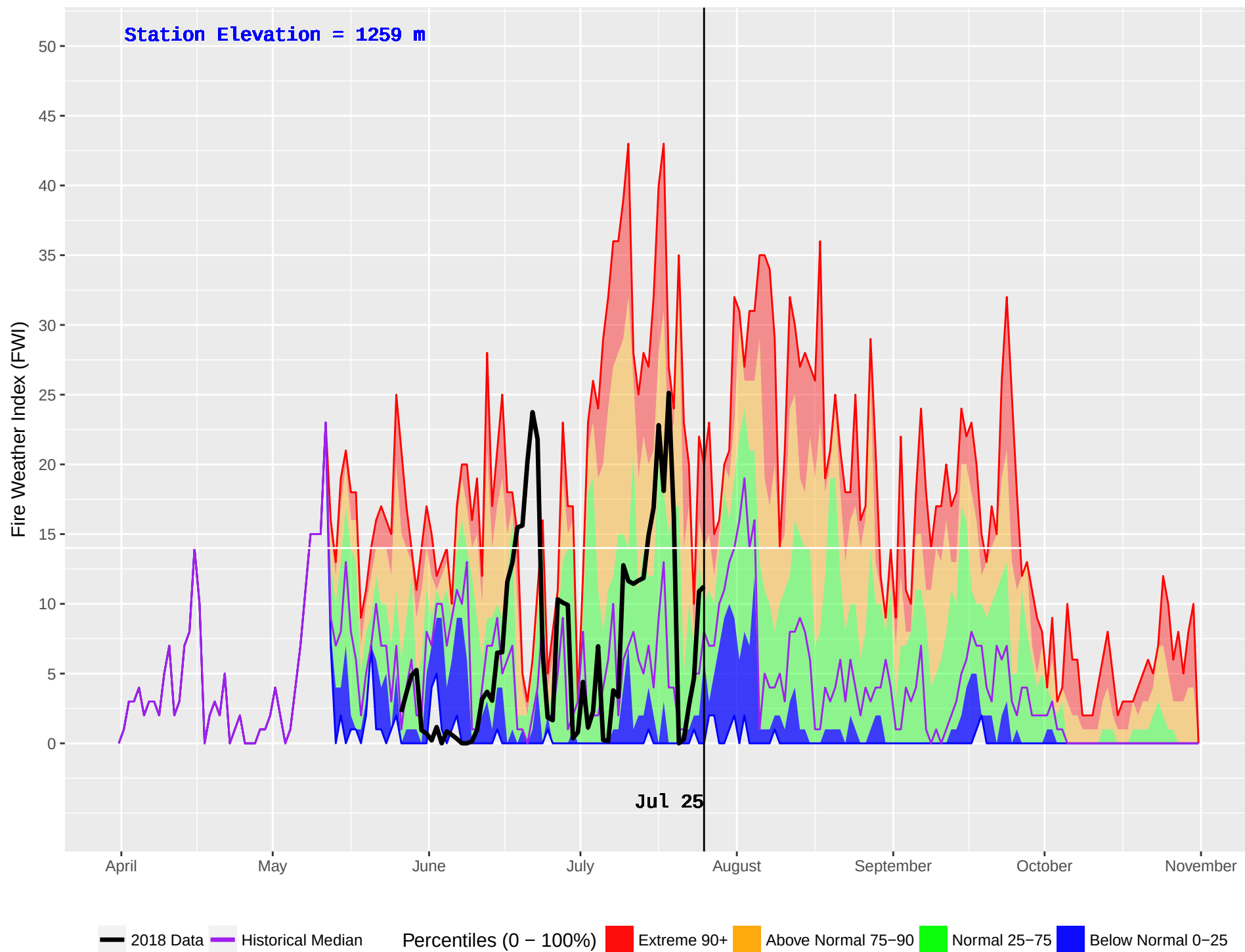
PARROTT (183) : Historical (1995–2016) and Current (2018) Noon Fire Weather Index (FWI)
