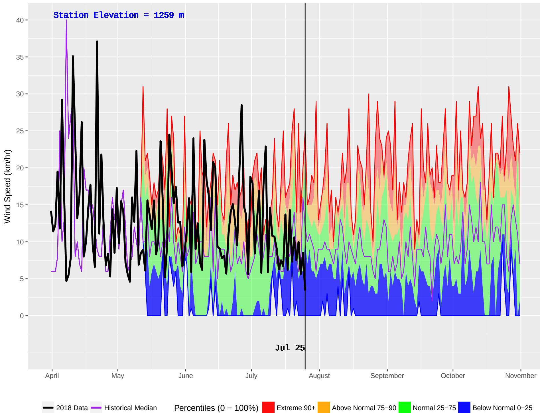
PARROTT (183) : Historical (1995–2016) and Current (2018) Noon Wind Speed
