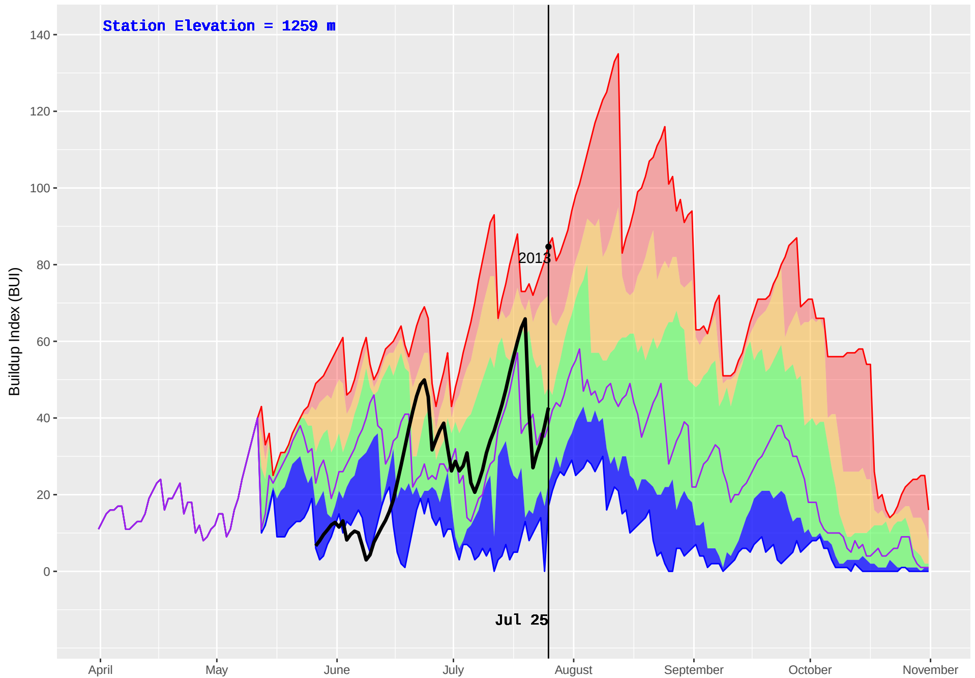
PARROTT (183) : Historical (1995–2016) and Current (2018) Noon Buildup Index (BUI)
