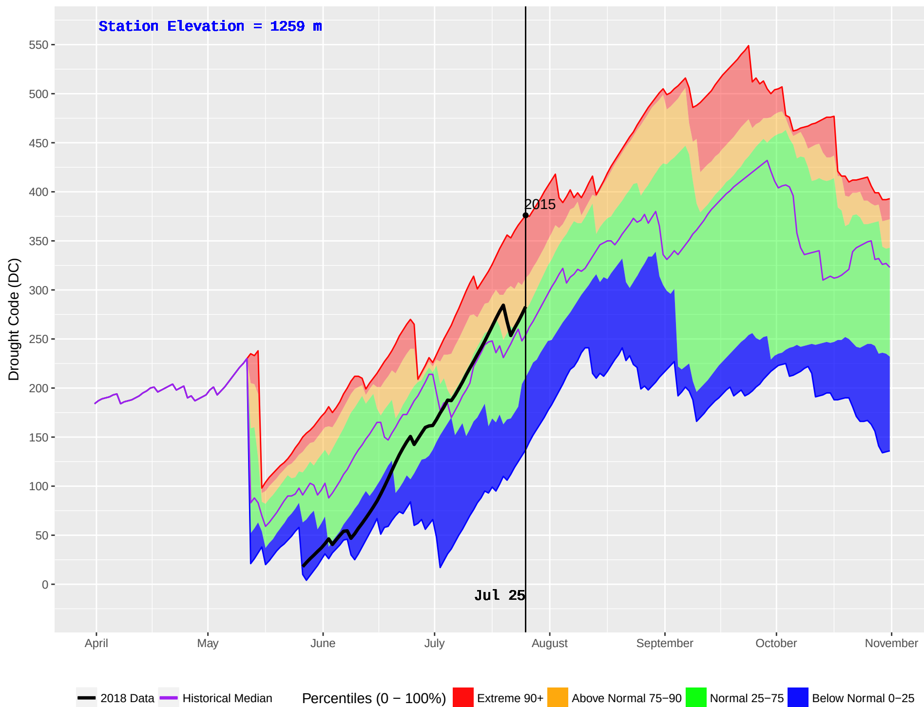
PARROTT (183) : Historical (1995–2016) and Current (2018) Noon Drought Code (DC)
