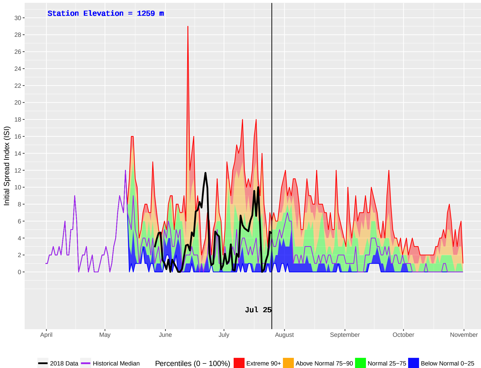
PARROTT (183) : Historical (1995–2016) and Current (2018) Noon Initial Spread Index (ISI)
